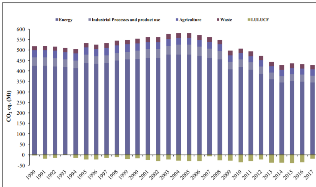
Figure 2.2 Greenhouse gas emissions and removals from 1990 to 2017 by sector (Mt CO 2 eq.)
